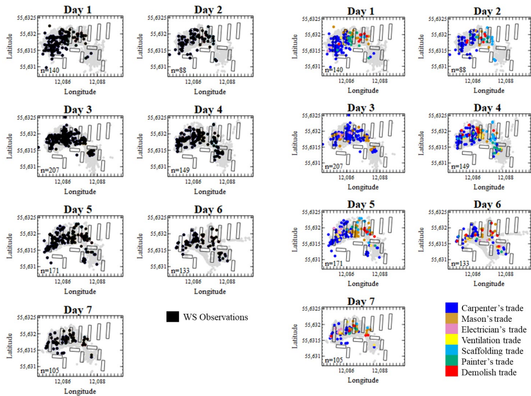
Figure 6: (a) Location of each observation; (b) Trade classification of each observation
