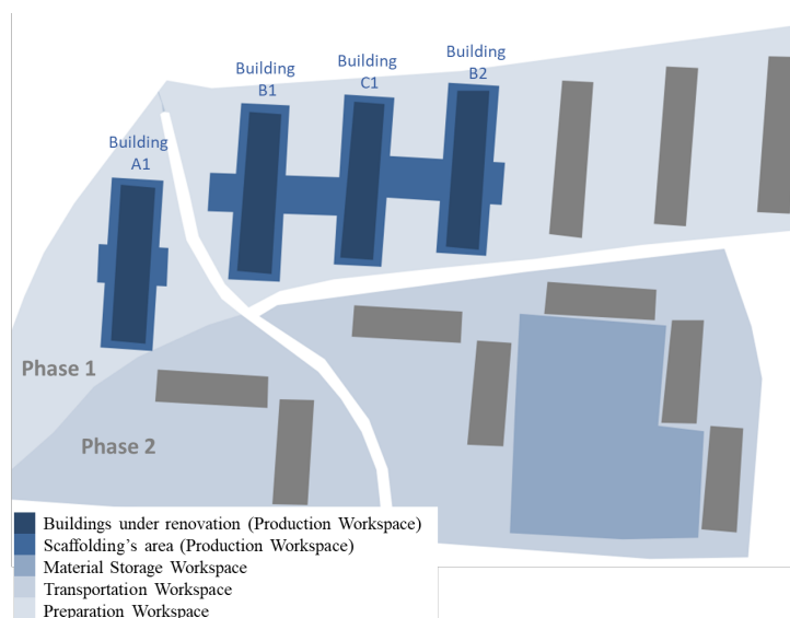
Figure 1: Job site layout
